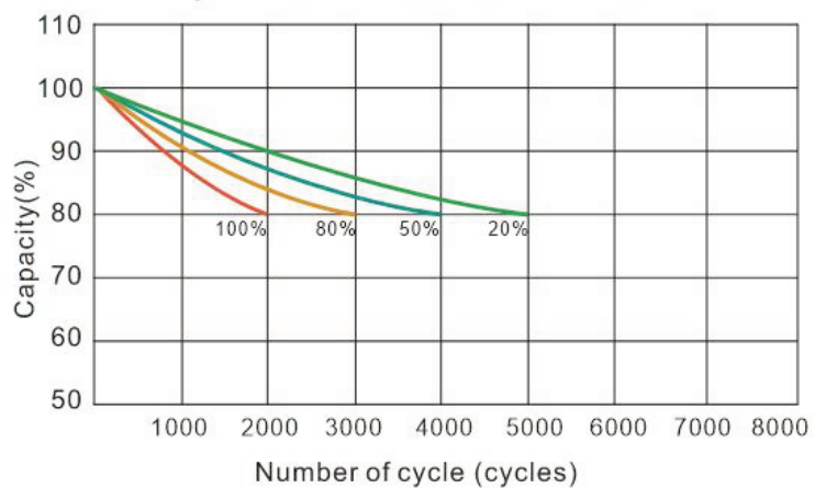
Cycle life with DOD at 25°C, 0.5C
