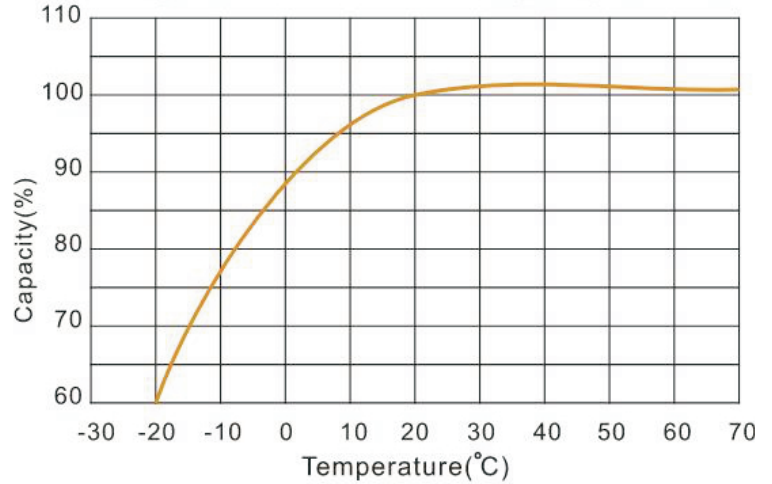
Temperature effects on capacity at 0.5C
